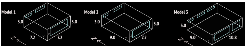
Figure 2. The geometry of classrooms models.
